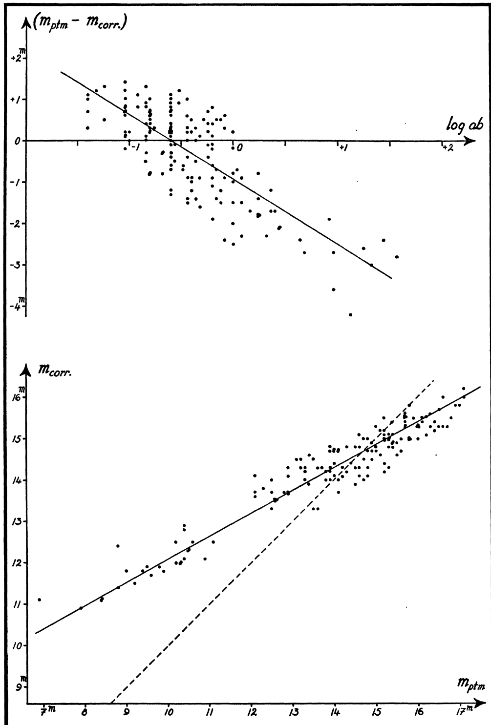
Fig. 13. Systematic deviations of the photometric magnitudes.
