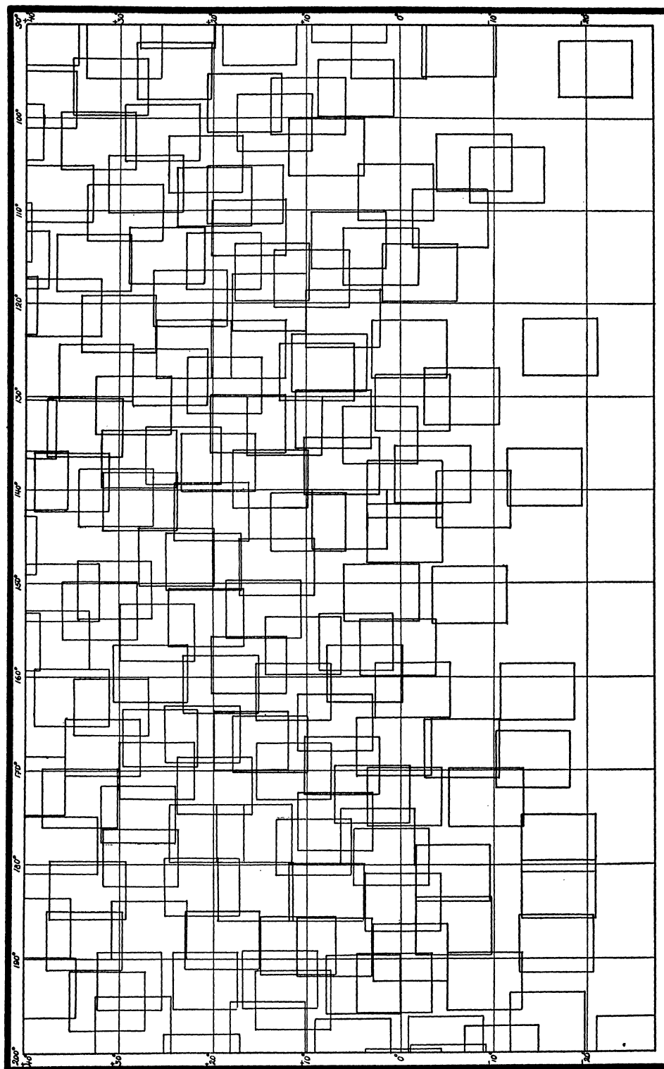
Fig. 37. Equatorial distribution of the plates used for the present investigation.
