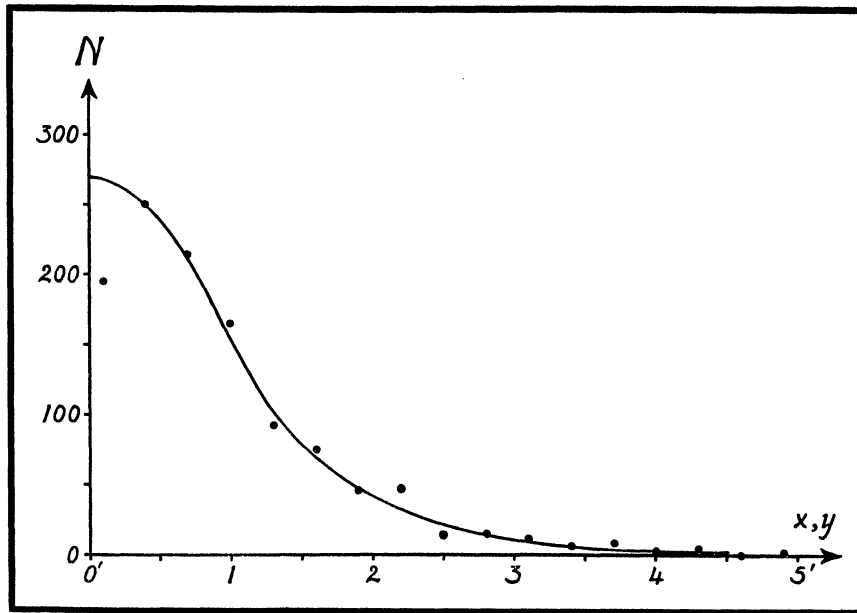
Fig. 33. Distribution of the apparent distances x and y .
