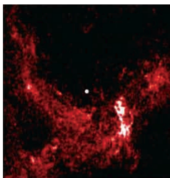
8 arcsec 1 light year
