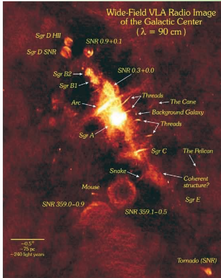
Figure 6. Big picture of the central region of the galaxy, the inner few hundred light years. (Image from NRAO/AUI N.E. Kassim)
