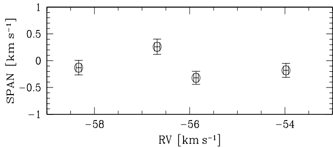
Fig. 5: The bisector span, giving the differences in radial velocities between top and bottom of a bisector, as a function of radial velocity, measured with HARPS .
