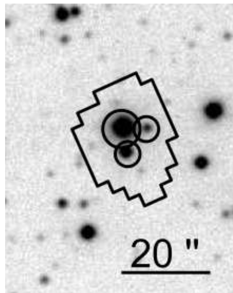
Fig. 3: A CCD image of the field around CoRoT-Exo-3, observed with the IAC80 telescope at a seeing with a FWHM of 1.4''. The largest circle indicates the CoRoT-Exo-3b host star, whereas the smaller circles below and to the right indicate contaminating stars that are 2.9 mag and 4.9 mag fainter, at distances of 5.6'' to the South and 5.3'' to the East, respectively. The irregular shape is the photometric mask used by CoRoT . Please note that the East is to the right on the figure.
