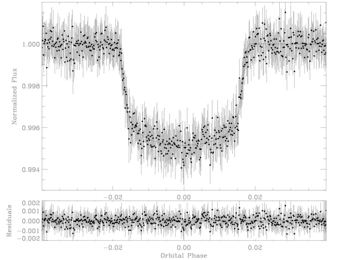
Fig. 2: The phase-folded light curve of the CoRoT-Exo-3b transit with the best fit solution overplotted (solid line). The residuals of the fit are plotted at the bottom of the figure. The rms error is 4.4094 \cdot 10^{-4} out of eclipse.
