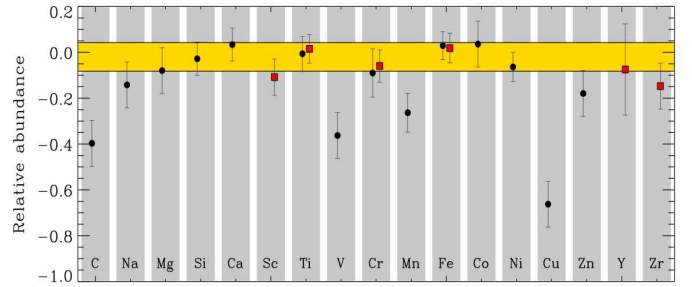
Fig. 7: Abundances of the elements measured in CoRoT-Exo-3. Black circles are for neutral elements and box symbols are used for ionized ones. The metallicity and the 1-\sigma uncertainty range are indicated by the horizontal yellow bar.
