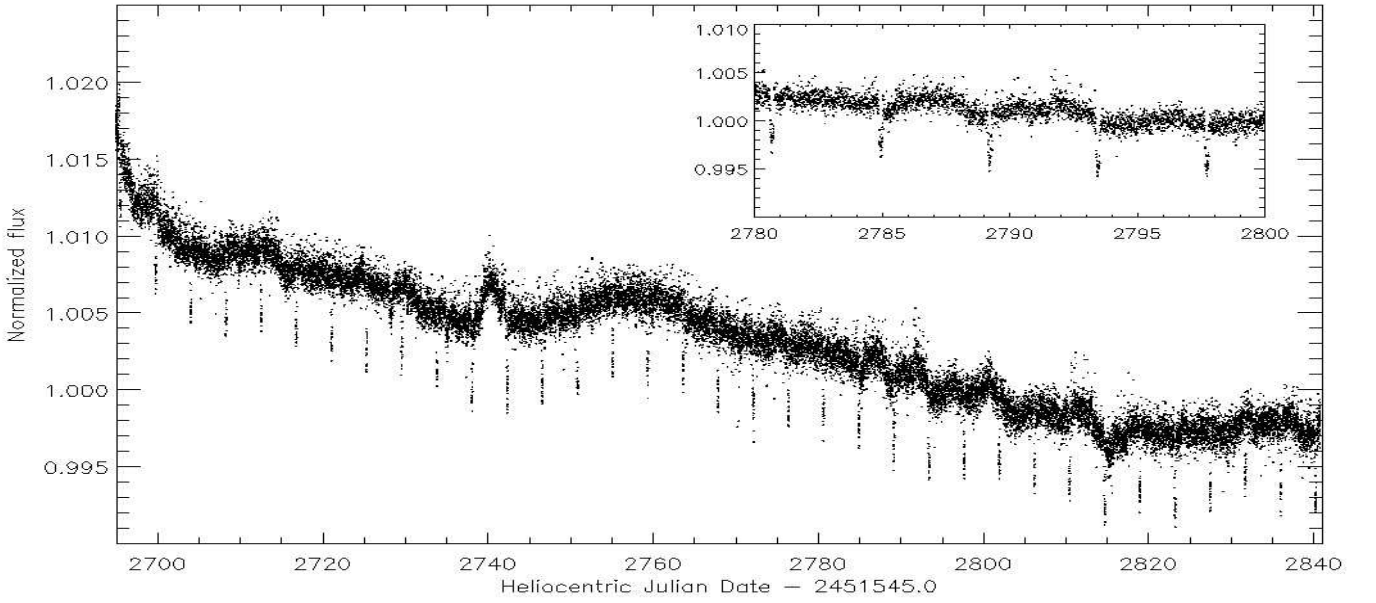
Fig. 1: The 152-days long CoRoT-Exo-3b reduced light curve, binned at a constant time sampling of 512 sec and normalized. The low activity level of the star is illustrated in the upper figure which displays a zoomed section of the light curve.
