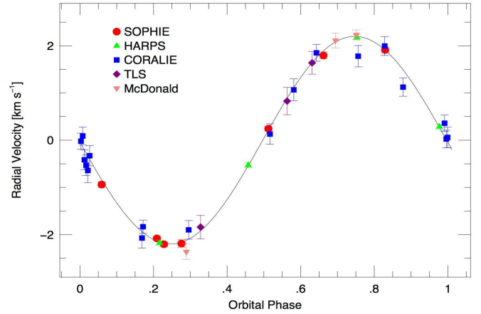
Fig. 4: The phase-folded radial velocity measurements from the different spectrographs used for the follow-up campaign, with the best fit solution over-plotted (solid line).
