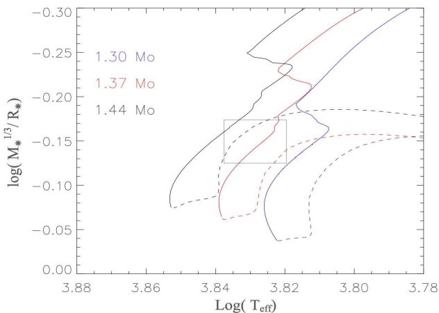
Fig. 9: Stellar evolutionary tracks from the STAREVOL models
