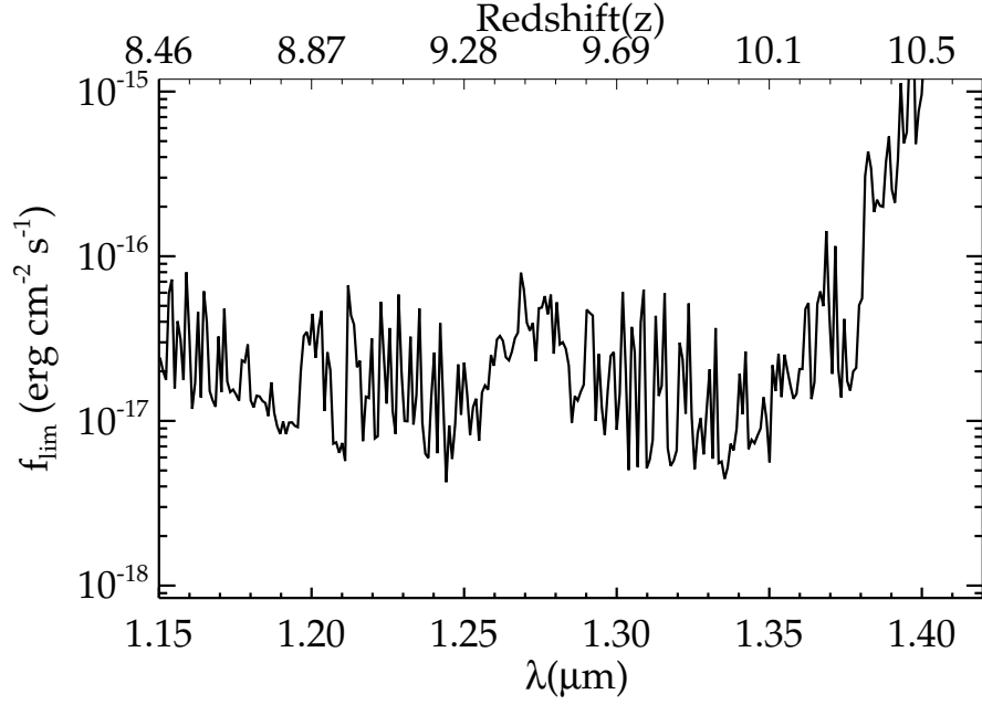
FIG. 3.— Limiting flux for detection of 5\sigma Lyman- \alpha emission line for a typical NIRSPEC J band exposure. The top axis denotes the redshift corresponding to observed Lyman- \alpha at the wavelength along the bottom axis. OH bands lie throughout the J-band spectrum, significantly increasing the limiting flux at those wavelengths. The widest band occurs in the middle of the spectrum at \simeq 1.26 - 1.28\mu m .
