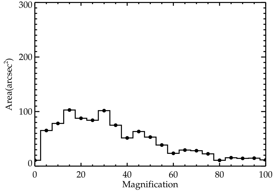
FIG. 5.— Distribution of lensing magnification across our total survey area. The median magnification across our survey area is \simeq 20 , about a factor of 2 larger than in a similar optical spectroscopic lensing survey (Santos et al. 2004) (see §3.4 for explanation). A non-negligible fraction of each slit is magnified by larger than this factor.
