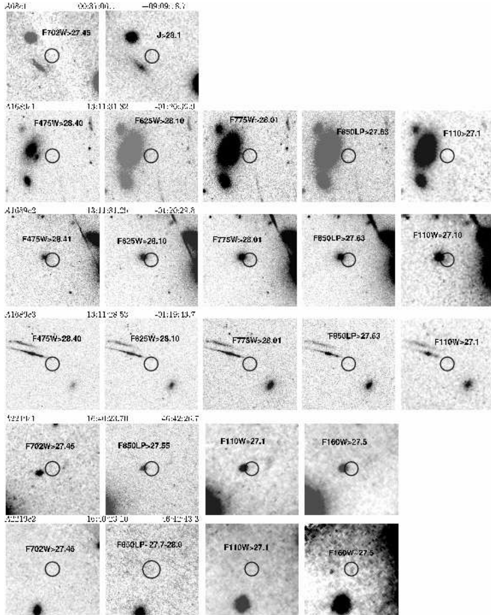
FIG. 8.— Deep broadband images of the locations of the candidate J-band emission features. None of the candidates have definitive detections in the optical; although A2219c2 is very marginally detected in the z'_{F850LP} and H_{F160W} bands. Three of the candidates are located within several arcseconds of brighter objects (A2219c1, A1689c1, and A1689c2); however in both cases, our registration is known to sufficient precision to rule out the possibility that the J-band emission features emanate from the bright objects. The lack of detection in very deep near-IR images suggests that if these candidates are at z \simeq 9 , then their rest-frame UV continuum emission is very faint.
