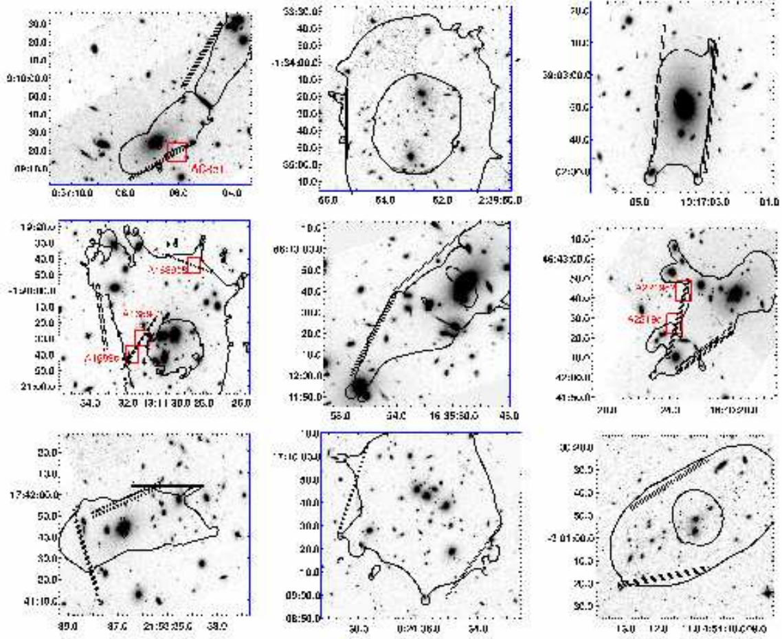
FIG. 2.— Survey clusters, with survey area and lensing critical curves. For each cluster, superposed on the HST /WFPC2 image are slit positions observed with NIRSPEC and the critical lines for a source at z = 8 (dotted lines). The solid curves bound areas where the magnification provided to z = 8 background sources exceeds a factor of 10. From left to right and top to bottom are Abell 68, Abell 370, Abell 963, Abell 1689, Abell 2218, Abell 2219, Abell 2390, CL 0024, MS 0451.
