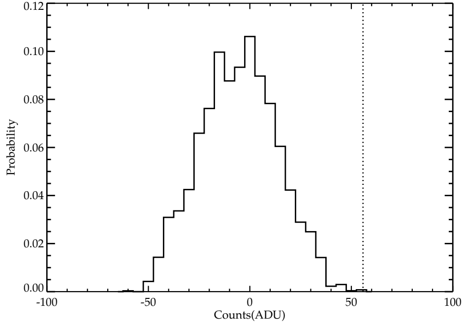
FIG. 7.— Normalized histogram of summed flux in randomly placed apertures in clean regions of sky-subtracted spectra. The dotted line represents value of a typical candidate Lyman- \alpha emitter. The frequency of features with fluxes on par with the candidates is 0.02%, consistent with a \simeq 4\sigma detection assuming a Gaussian distribution of noise.
