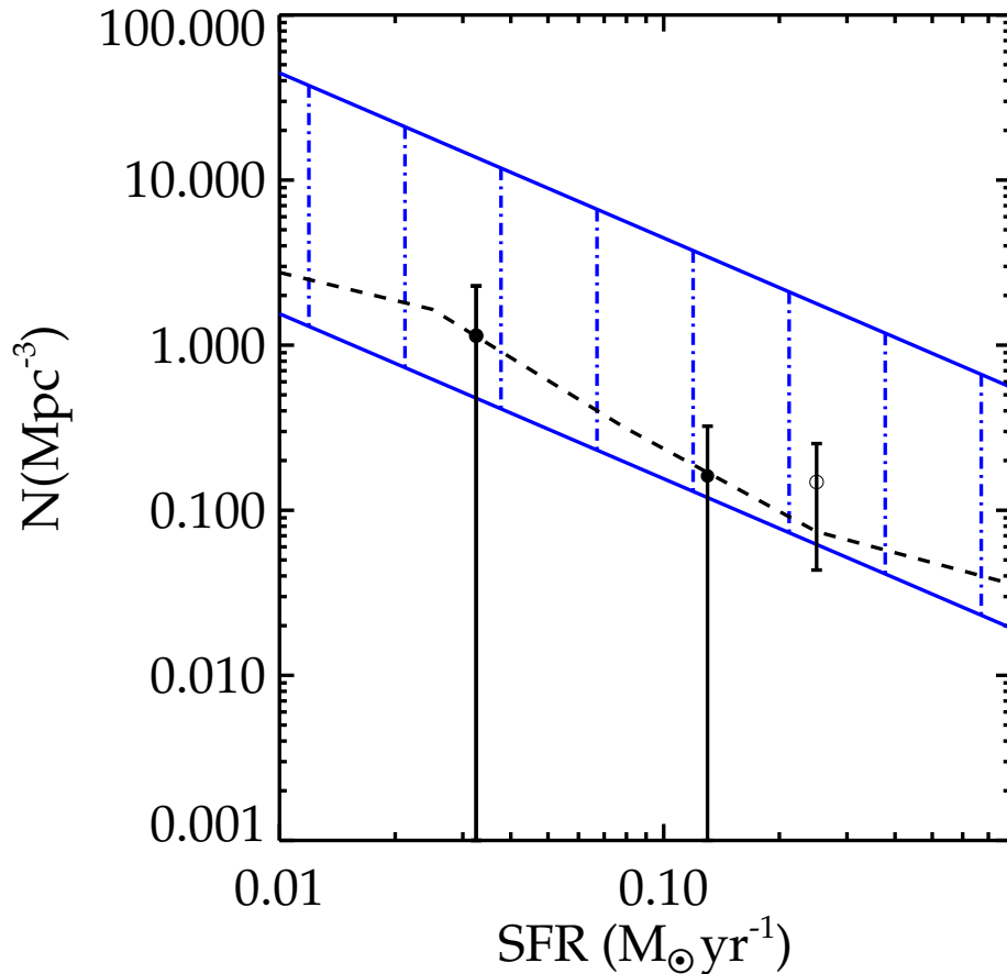
FIG. 12.— Abundance of sources required for reionization assuming a single population of star-forming galaxies dominates the process (blue swath) compared the observed abundances (a) if all the candidates are real (open circles), (b) two of the candidates are real (solid circles), or (c) if none of the candidates are real (dotted line). The abundance constraints for case a and case b are identical for the two lowest luminosity bins plotted in the figure. The range for the abundance of sources required for reionization is determined assuming f_c=0.5 , \Delta t_{reion}=575 Myr, and B=10 for the lower locus of points and f_c=0.02 , \Delta t_{reion}=250 Myr, and B=5 for the upper locus of points. If two or more of the candidates are real, then it appears that intrinsically faint galaxies may play a dominant role in the reionization of neutral hydrogen.
