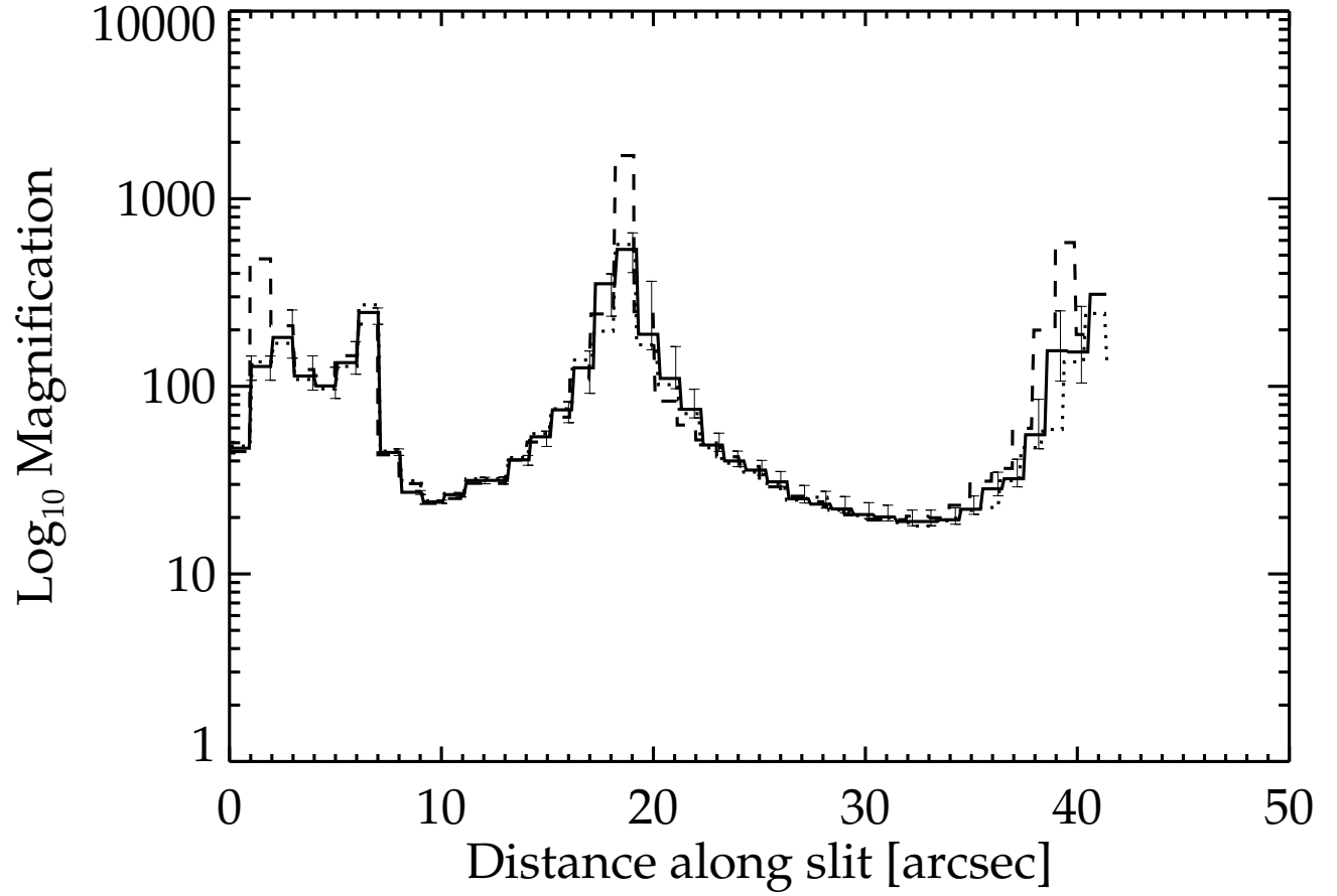
FIG. 4.— Lensing magnification provided to background sources as a function of NIRSPEC slit position and redshift. This figure shows the amplification at one of the slit positions along the critical line of Abell 2219. The solid line corresponds to the amplification provided to background sources at z=9 whereas the dotted and dashed line denotes that provided to sources at z=8.5 and 10.0 , respectively. The error in lensing magnification is plotted as a function of NIRSPEC slit position for sources at z=9 . The error does not vary significantly as a function of source redshift. Even allowing for uncertainty in the mass model, the magnification is still very high across the entire slit.
