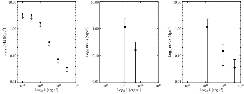
FIG. 11.— Constraints on number density of 8.5 < z < 10.2 sources with Lyman- \alpha luminosity brighter than L . Left: The 5\sigma upper limit to the abundance of low luminosity Lyman- \alpha emitters is presented assuming none of our candidate Lyman- \alpha emitters is real. Middle: The cumulative abundance of Lyman- \alpha emitters if two of the candidates (A68c1 and A2219c1) are real. Right: The cumulative abundance of Lyman- \alpha emitters assuming each of the six candidates is a Lyman- \alpha emitter. If even one candidate is real, the inferred abundance of low luminosity Lyman- \alpha emitters at z \simeq 9 would be very high.
