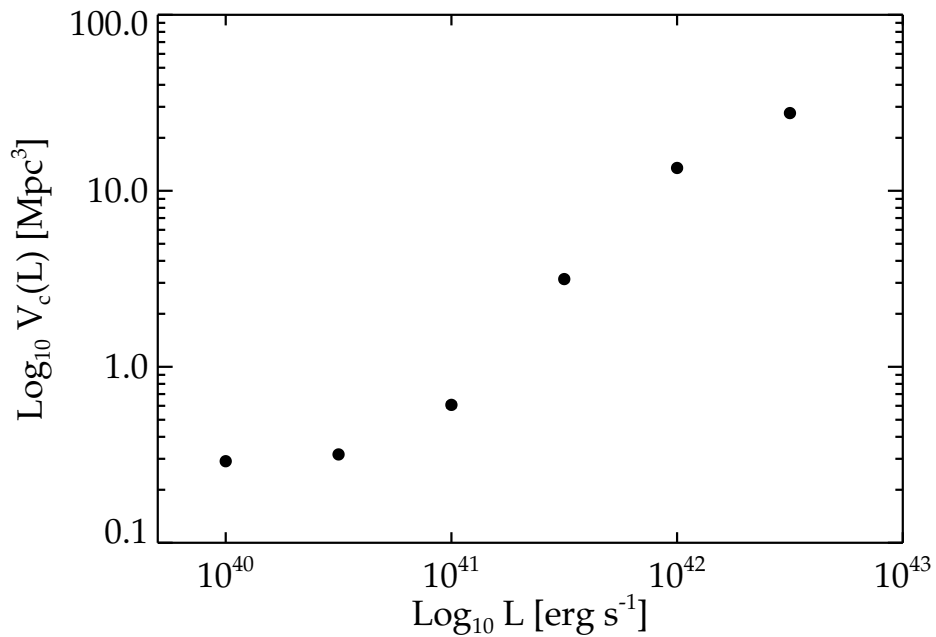
FIG. 10.— Survey volume (comoving) sensitive to sources with Lyman- \alpha luminosity L . The volumes observed are very small as a result of the small area of the spectroscopic slit and the decrease in survey area resulting from gravitational lensing.
