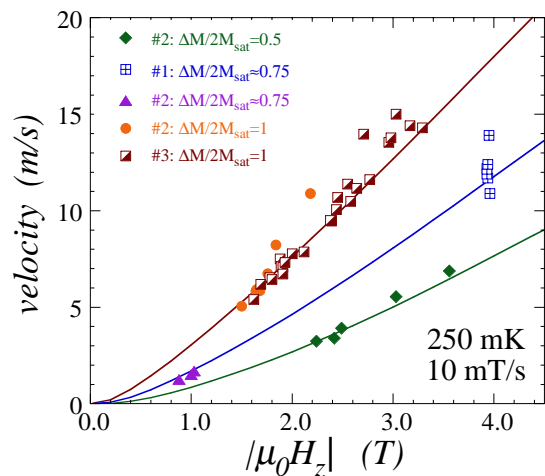
FIG. 4: Velocity of propagation of avalanches versus the magnetic field at which the avalanches occurred (samples are identified by number). ZFC denotes data obtained for the sample cooled in the absence of a magnetic field. From top to bottom, the curves are fits obtained for \Delta M / 2M_{sat} = 1, 0.75 and 0.5 (see text).
