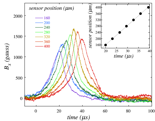
FIG. 3: Signals recorded by seven equally spaced Hall sensors situated near the center of sample 1 during an avalanche triggered at 4 T. The left (right) trace corresponds to the top (bottom) sensor (see Fig. 1). Sensor positions are measured relative to the top of the sample, with the center at \approx 320 \mu\text{m} . The inset shows sensor position versus the time at which the sensor recorded peak amplitude. A straight line fit yields a constant velocity of propagation of 12 m/s.
