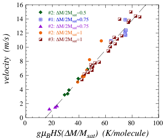
FIG. 5: Velocity of propagation of avalanches versus energy released per molecule. The line is drawn to guide the eye.
