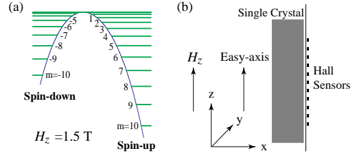
FIG. 1: (a) The potential energy function in a longitudinal magnetic field of 1.5 T; (b) Schematic diagram of a sample mounted on an array of Hall sensors used to detect B_x . Pronounced non-uniformity in magnetization during an avalanche generates large values of B_x .
