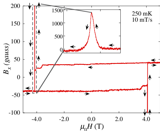
FIG. 2: Hysteresis loops for a single crystal of \text{Mn}_{12}\text{-ac} (sample 1). B_x was recorded by a Hall sensor situated about 80 \mu\text{m} above the middle of the sample. Steps due to quantum tunneling of the magnetization are observed, as well as a sharp spike in B_x associated with an avalanche, shown in the inset.
